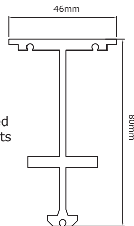
TRACK SECTION
